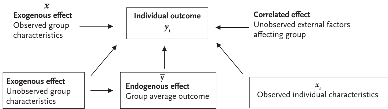
Figure 5. Estimation issues in social effects
